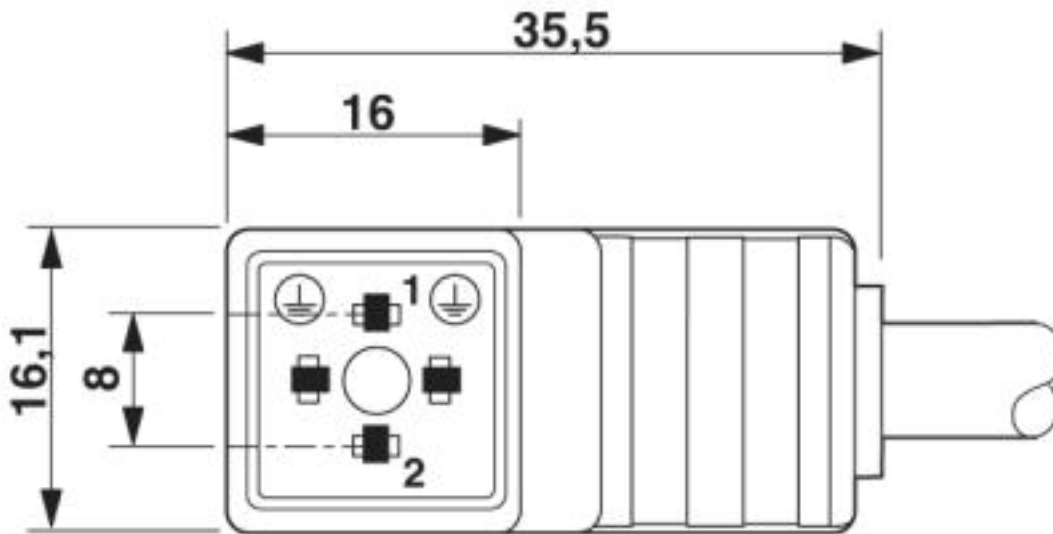
Dimensional drawing
