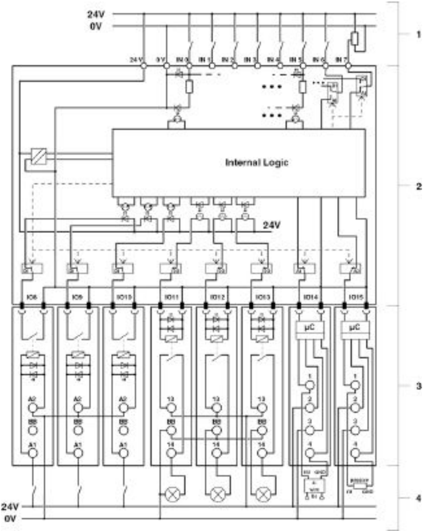
Circuit diagram
