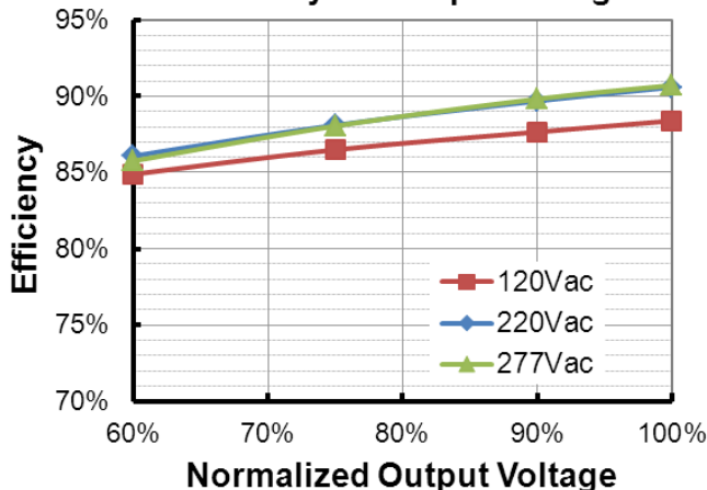
EUD-096S070BVA (I o =700mA) Efficiency vs. Output Voltage
