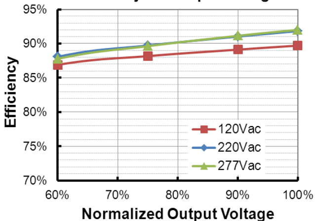
EUD-096S070BVA (I o =450mA) Efficiency vs. Output Voltage
