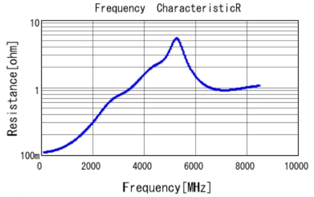
■ GCM0335C1E750FA16 R DC0V, 25degC
