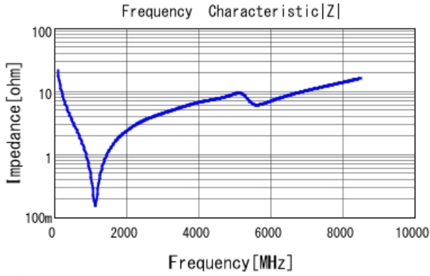
■ GCM0335C1E750FA16 |Z| DC0V, 25degC
