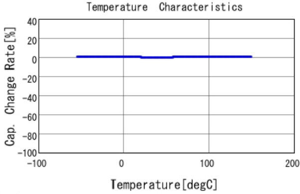
■ GCM1555G1H201FA16 C-Temp. capchange, DCOV, AC1Vrms
