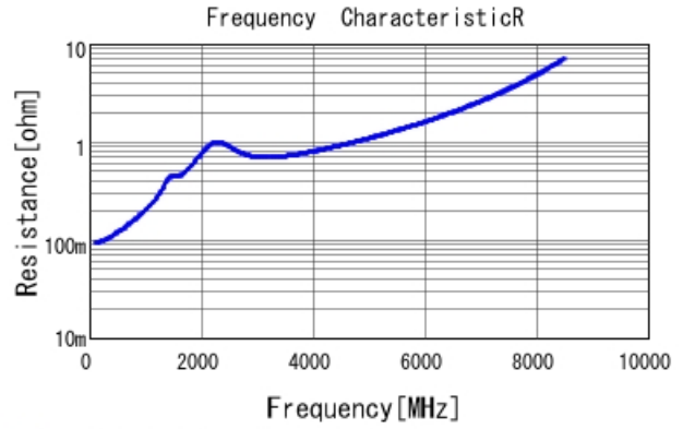
GCM1555G1H201FA16 R DCOV, 25degC
