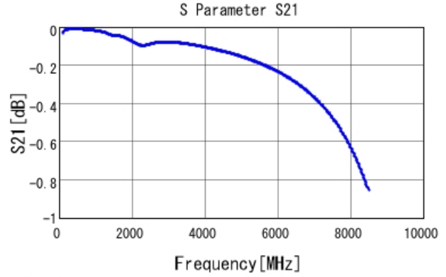
■ GCM1555G1H201FA16 S21 DCOV, 25degC
