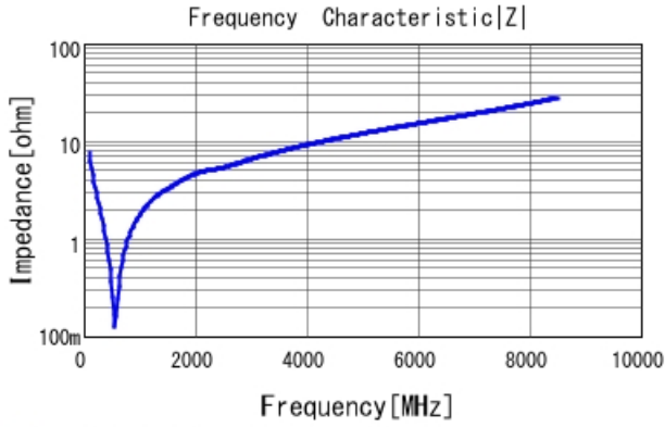
GCM1555G1H201FA16 |Z| DCOV, 25degC
