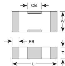
Dimensional View
