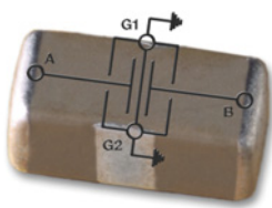
Equivalent Circuits
