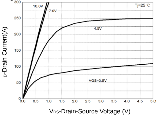
Figure 5: Output Characteristics
