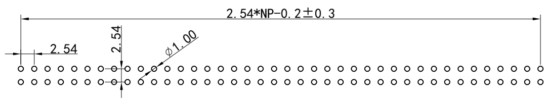
RECOMMENDED PCB LAYOUT COMPONENT SIDE VIEW
