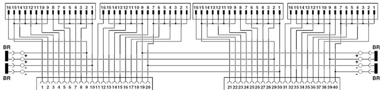
Circuit diagram
