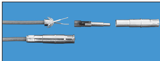
Size 8 RCT (Reduced Component Twinax) Contact (Also available in Size 10)
