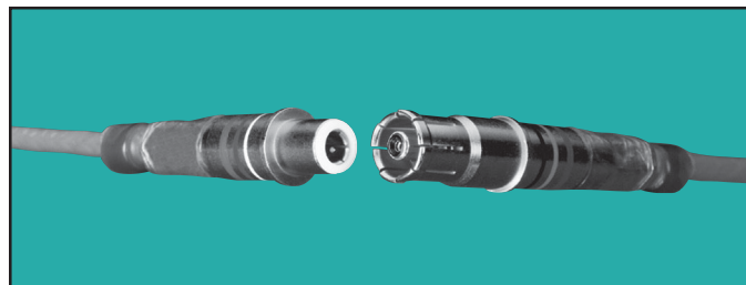
Size 8 Concentric Twinax Contacts Qualified to M39029/90 and /91 (Also available in Size 12)
