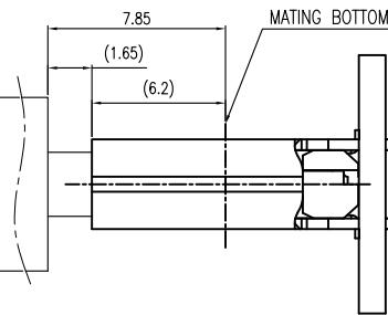
MATED CONDITION (REF)
