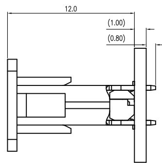
CAP ASSEMBLY AND MOUNTING CONDITION (REF)
