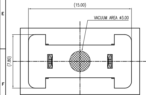
CAP ASSEMBLY AND MOUNTING CONDITION (REF)
