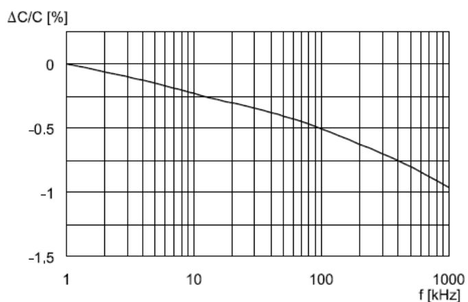
Capacitance change vs. frequency (Room temperature)
