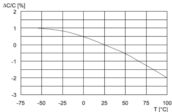
Capacitance change vs. temperature at 1kHz
