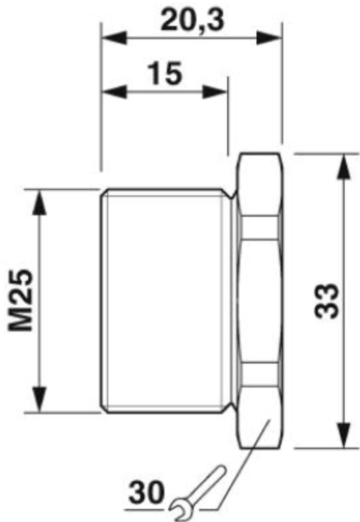
Dimensional drawing
