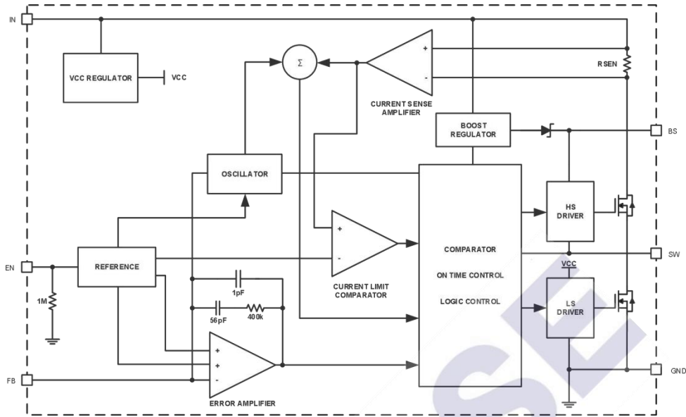
Figure 2. U0218/9 Block Diagram
