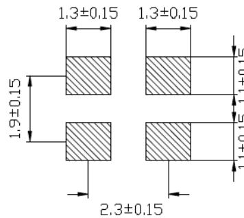
LAND PATTERN<REFERENCE>
