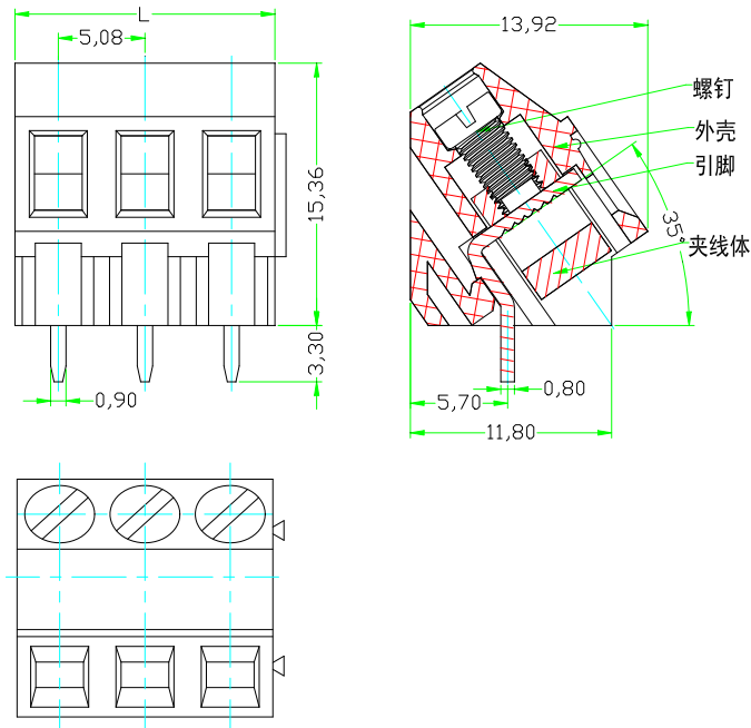
外形尺寸 (Shape Dimension)
