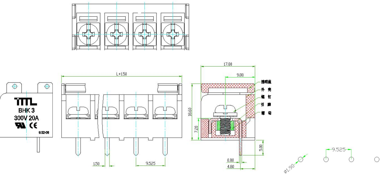
外形尺寸 (Shape Dimension)
