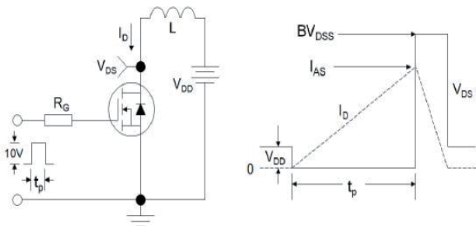
Figure 3: Unclamped Inductive Switching Test Circuit & Waveforms
