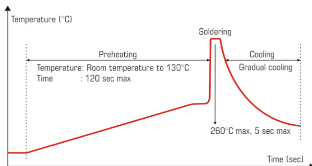
Fig.: Wave-soldering temperature-time profile to recommend
