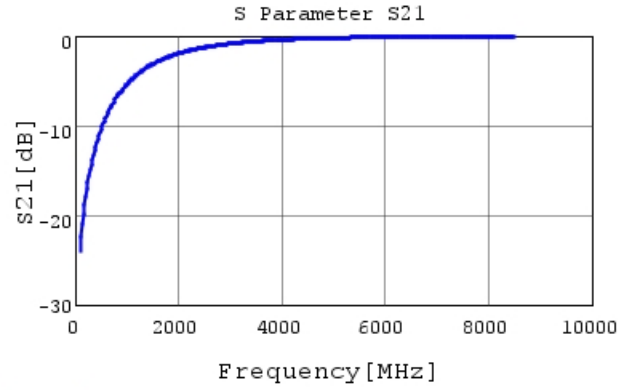
GCM1555C1H1R0JA16 S21 DCOV, 25degC
