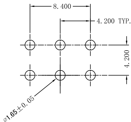
Recommened PCB Layout
