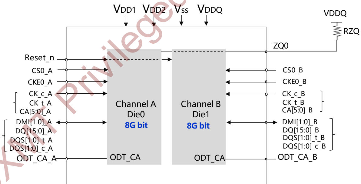
Figure 2-4 Dual-Die, Dual-Channel, Single-Rank Package Block Diagram (2GB x32 I/O)
