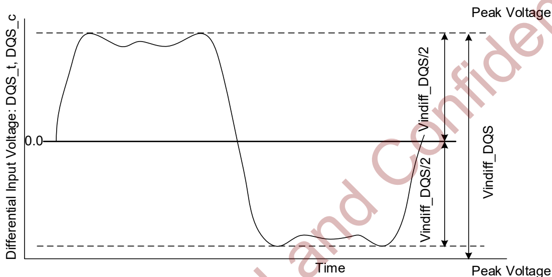
Figure 5-17 DQS Differential Input Voltage
