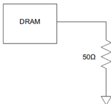
Figure 5-23 Driver Output Reference Load for Timing and Slew Rate
