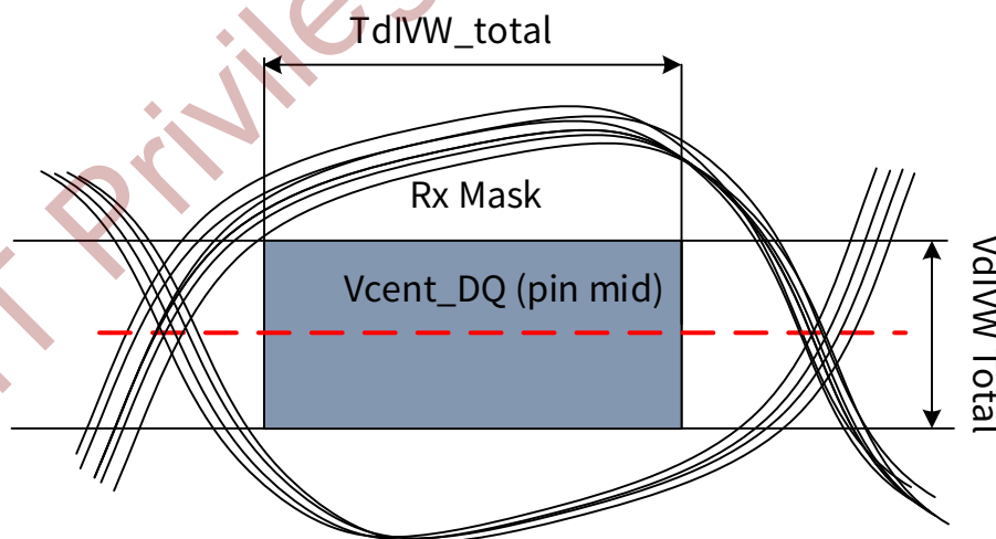
Figure 8-34 DQ Receiver(Rx) Mask
