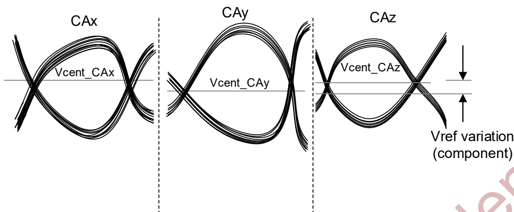
Figure 8-28 Across Pin VREFCA Voltage Variation
