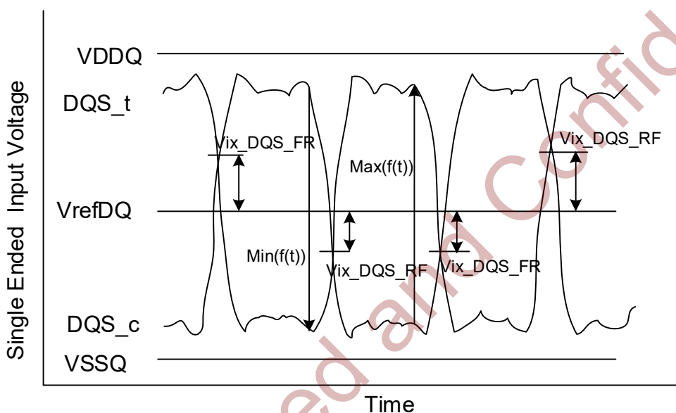
Figure 5-21 Vix Definition (DQS)
