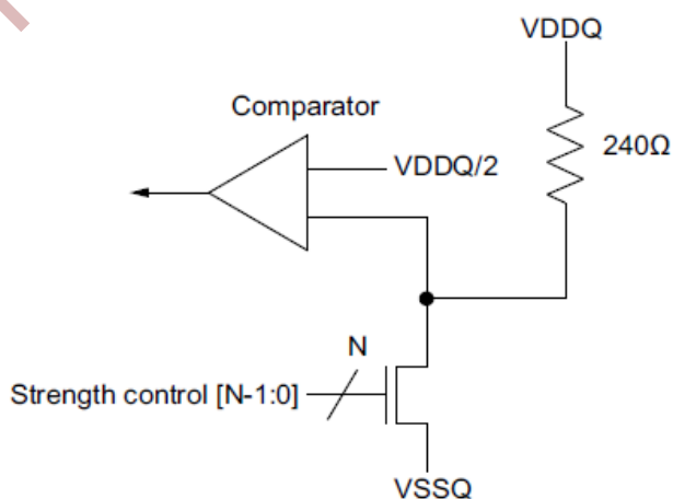
Figure 5-25 Pull-down Calibration
