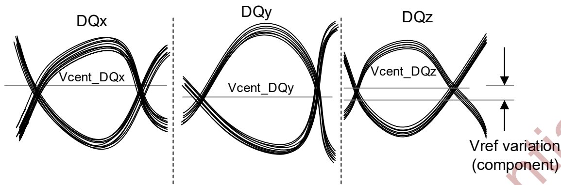
Figure 8-35 Across Pin Vref DQ Voltage Variation
