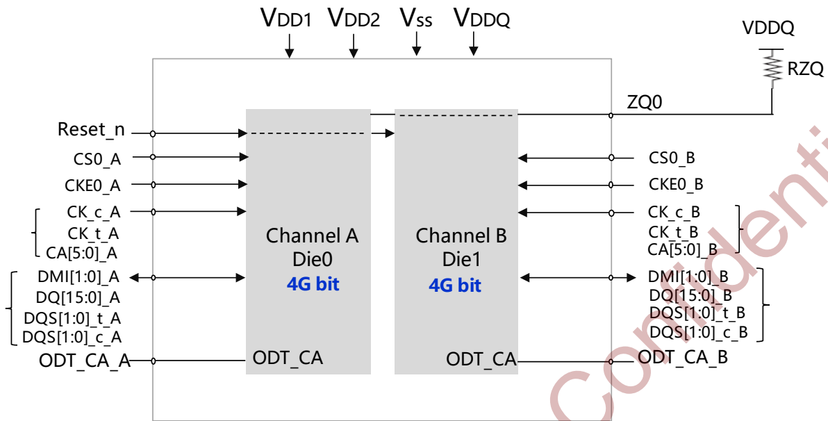
Figure 2-3 Dual-Die, Dual-Channel, Single-Rank Package Block Diagram (1GB x32 I/O)
