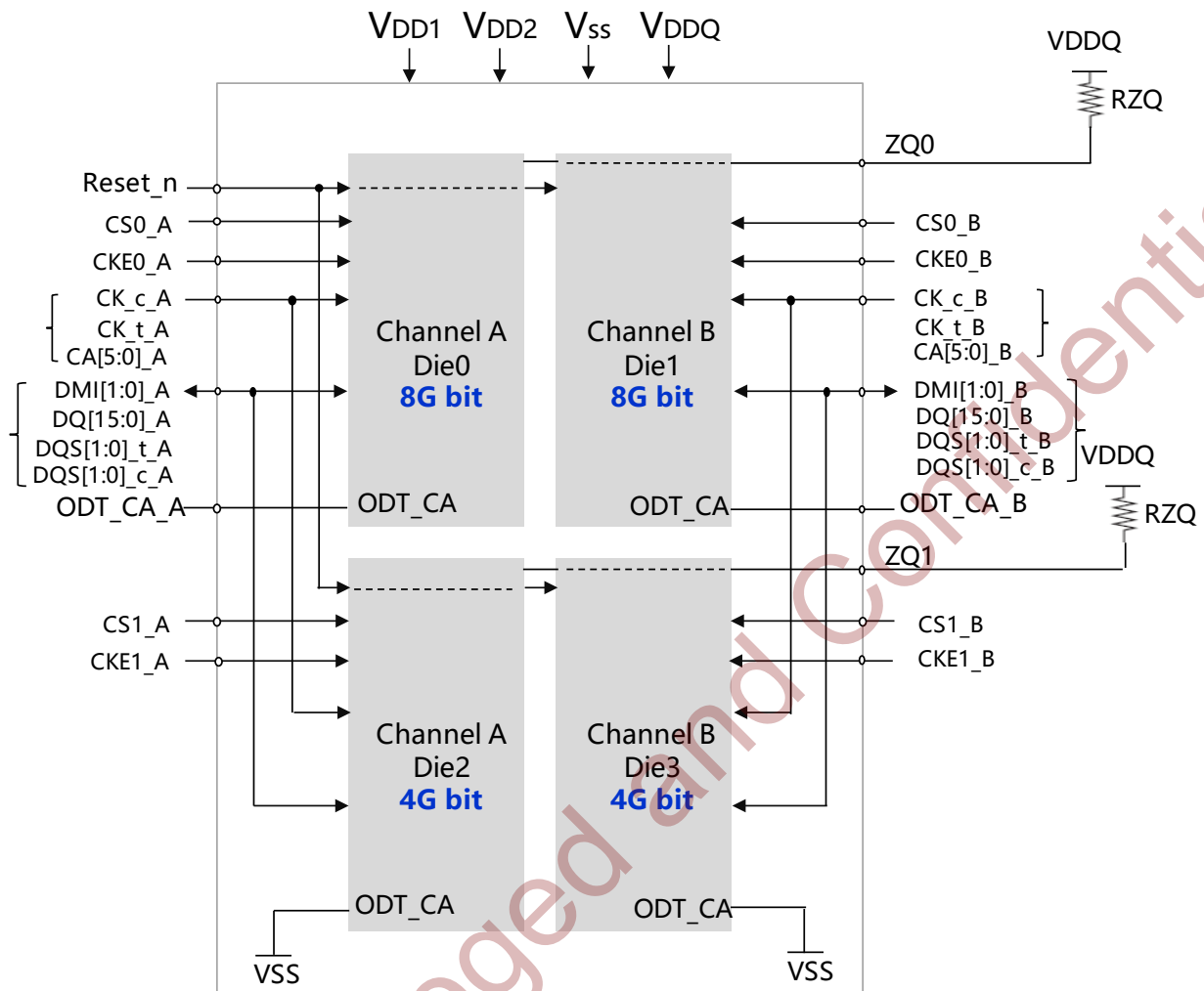
Figure 2-5 Quad-Die, Dual-Channel, Dual-Rank Package Block Diagram (3GB x32 I/O)
