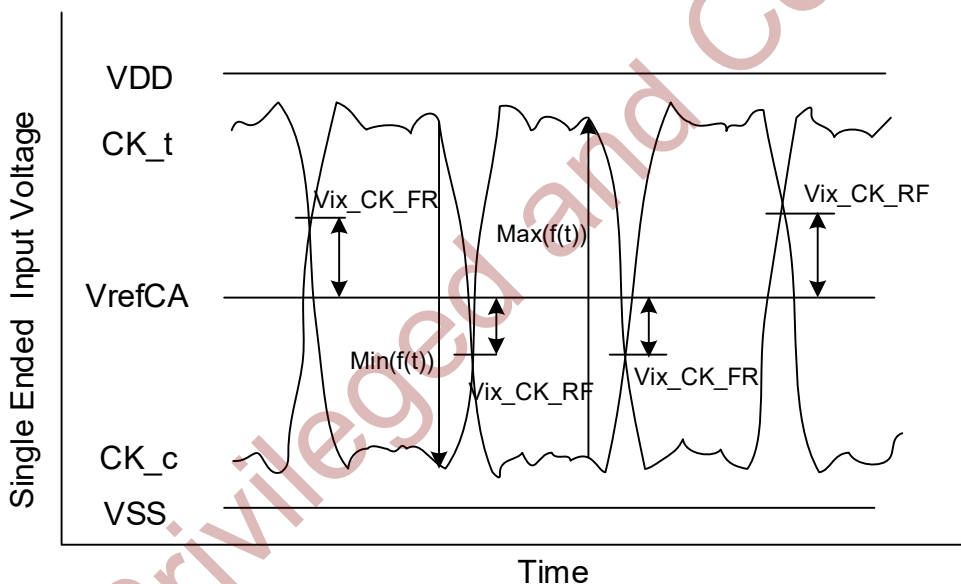
Figure 5-16 Vix Definition (Clock)
