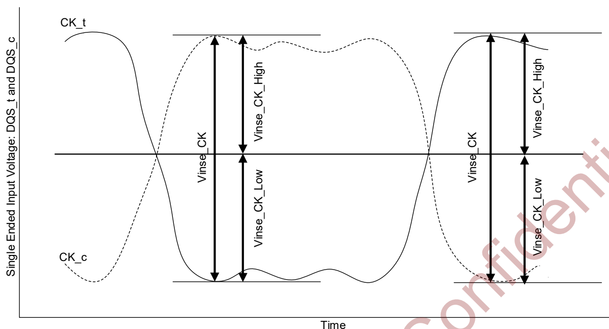
Figure 5-14 Clock Single-Ended Input Voltage
