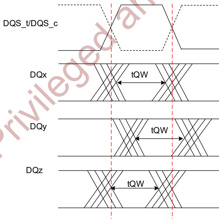
Figure 8-33 Read Data Timing t_{QW} Valid Window Defined per DQ Signal
