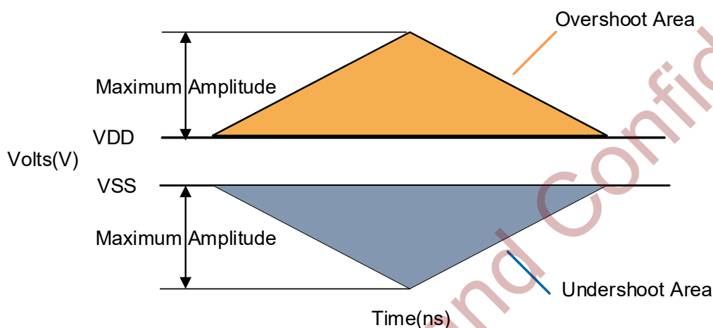
Figure 5-11 AC Overshoot and Undershoot Definition for Address and Control Pins
