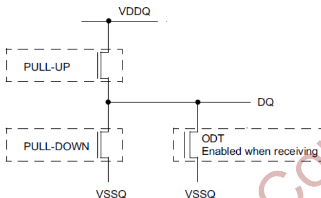
Figure 5-24 LVSTL I/O Cell
