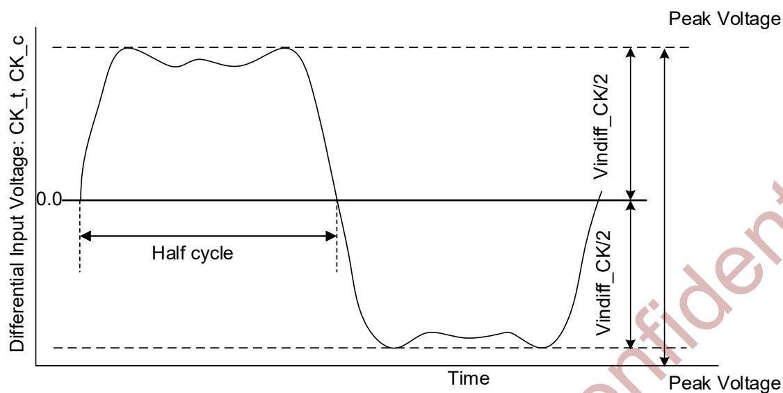
Figure 5-12 CK Differential Input Voltage
