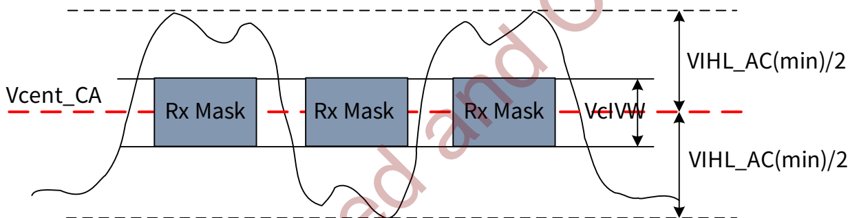
Figure 8-31 CA VIH_L_AC Definition (for Each Input Pulse)
