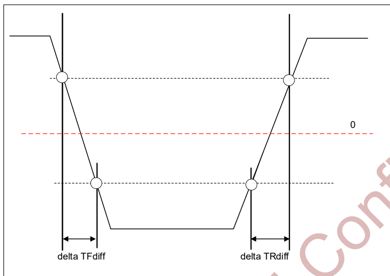
Figure 4-8 Differential Output Slew Rate Definition
