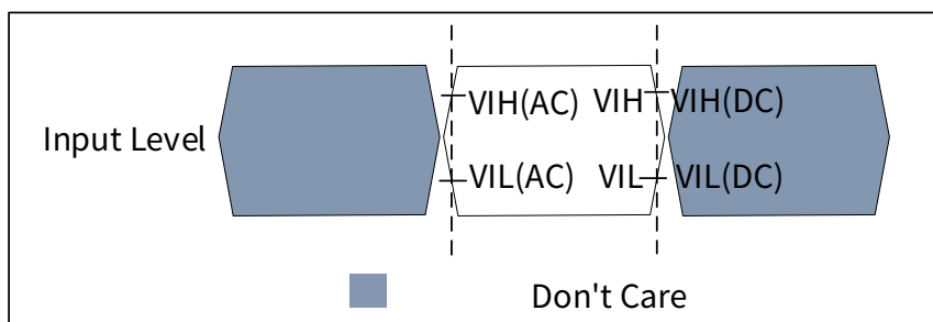
Figure 5-9 Input AC Timing Definition for CKE
