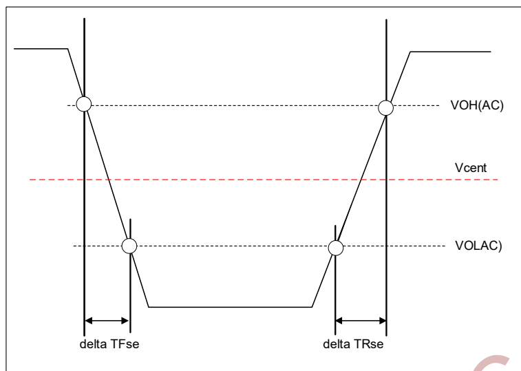
Figure 4-7 Single Ended Output Slew Rate Definition
