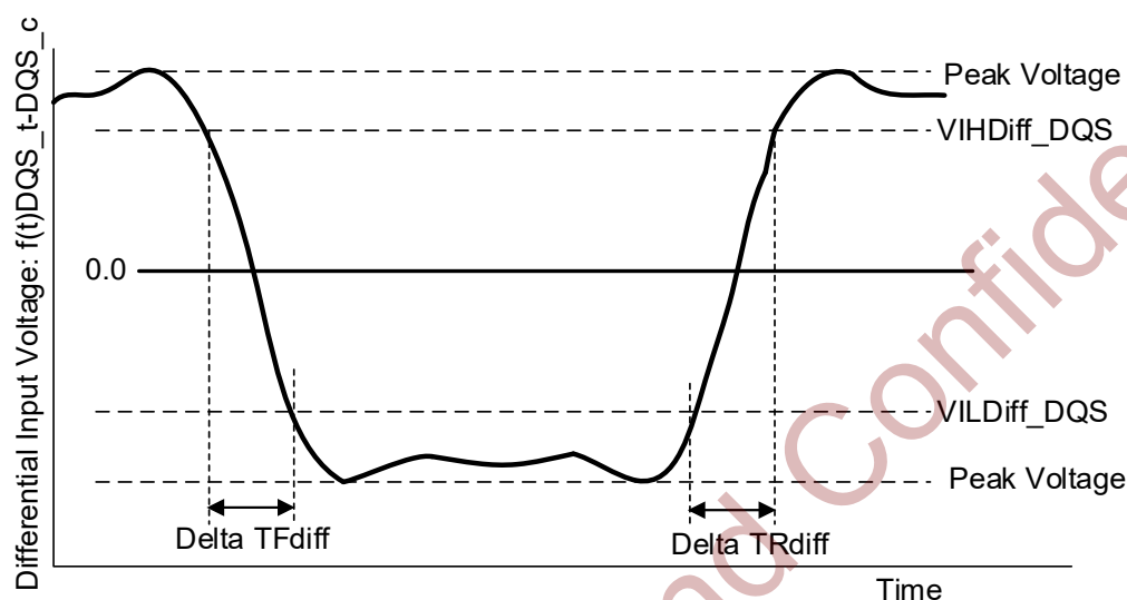
Figure 5-20 Differential Input Slew Rate Definition for DQS t , DQS c
