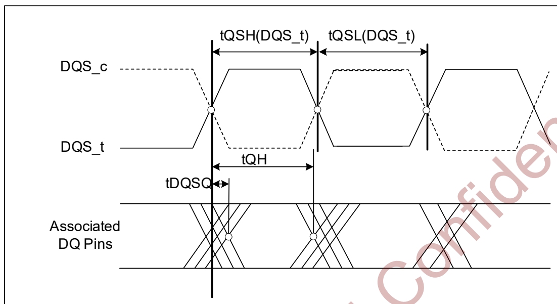
Figure 8-32 Read Data Timing Definitions t_{QH} and t_{DQSQ} across all DQ Signals per DQS Group
