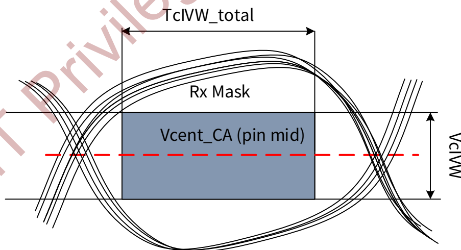
Figure 8-27 CA Receiver(Rx) Mask
