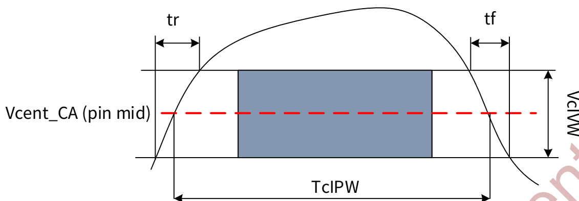
Figure 8-30 CA TcIPW and SRIN_cIVW definition (for each input pulse)
