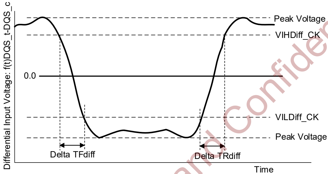
Figure 5-15 Differential Input Slew Rate Definition for CK t , CK c
