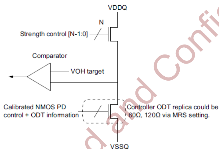
Figure 5-26 Pull-up Calibration
