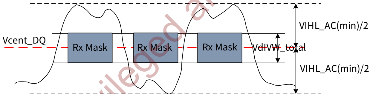
Figure 8-38 DQ VIH_L_AC definition (for Each Input Pulse)
