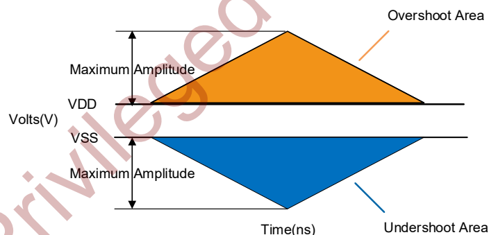
Figure 5-22 Overshoot and Undershoot Definition
