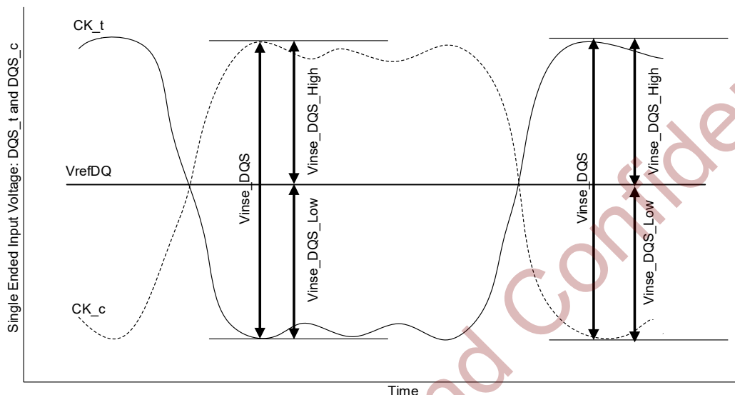
Figure 5-19 DQS Single-Ended Input Voltage
