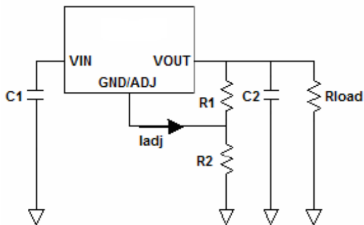
LD1117 adjustable output voltage
