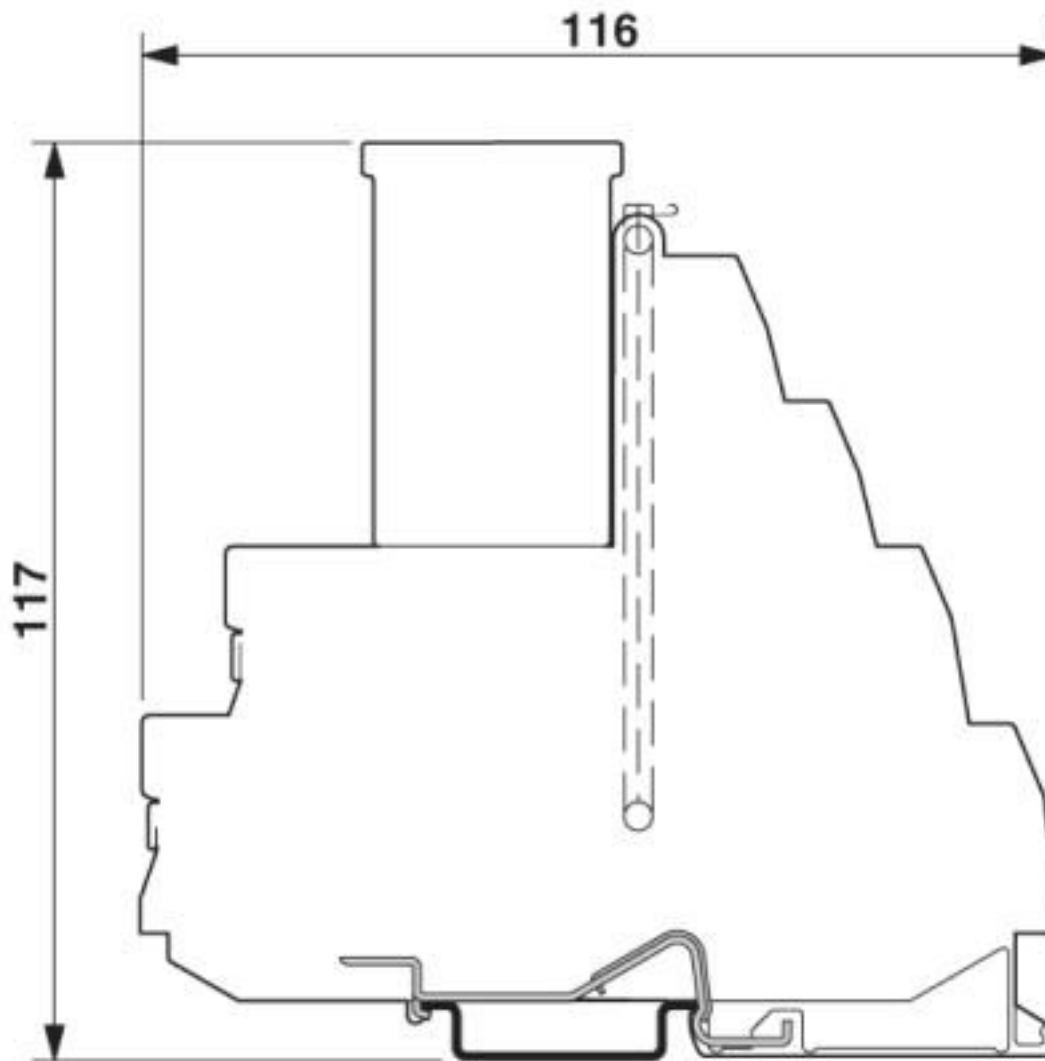
Dimensional drawing
