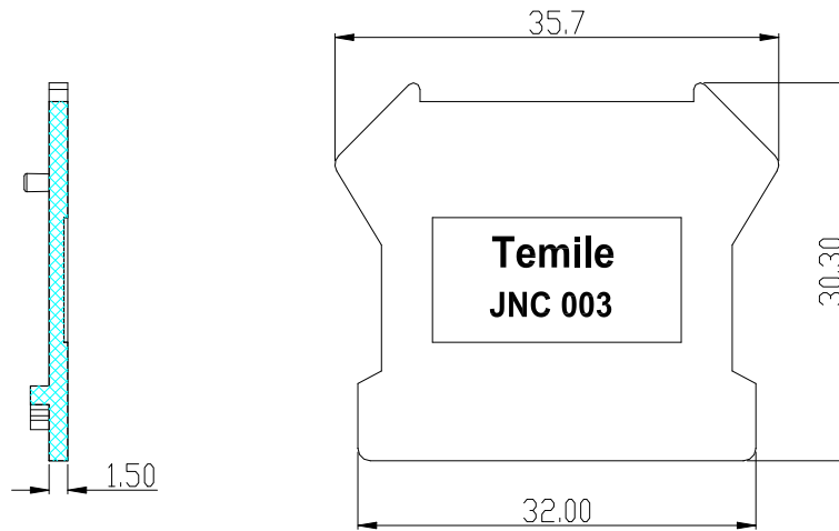
外形尺寸 (Shape Dimension)
