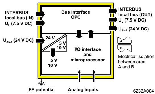
Figure 4 Electrical isolation of the single function areas
