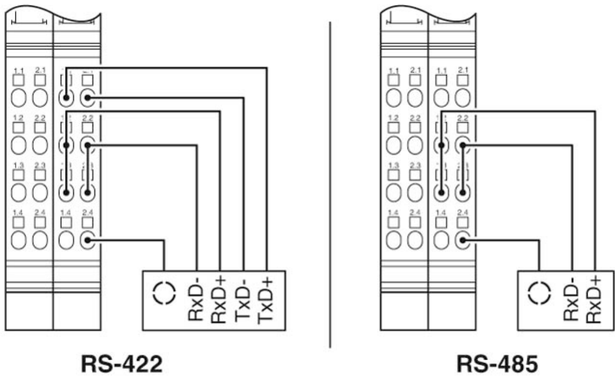
Connection diagram
