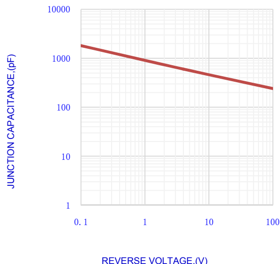
Fig.4-TYPICAL JUNCTION CAPACITANCE
