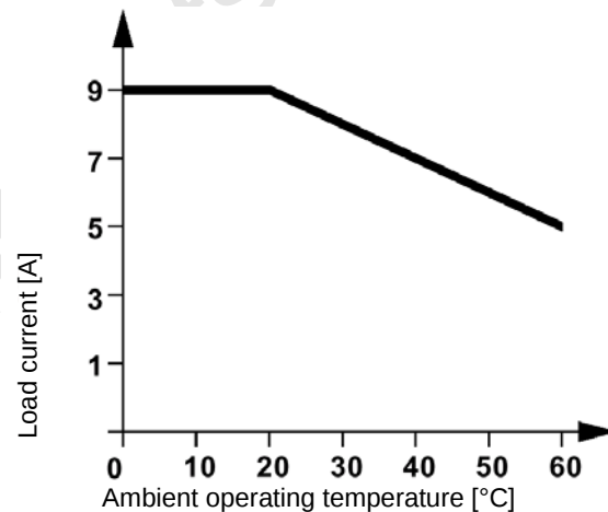
Figure 1 Load current depending on the ambient operating temperature
