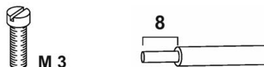
Figure 3 Connection data
