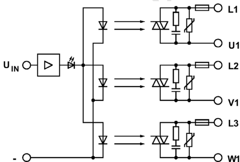
Figure 4 Block diagram
