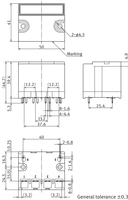
External dimensions
