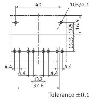
Recommended PC board pattern ( BOTTOM VIEW )
