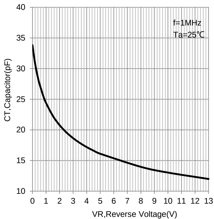
Capacitance
