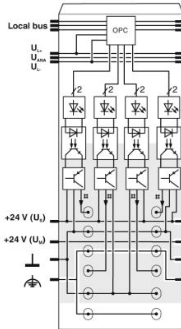
Block diagram
