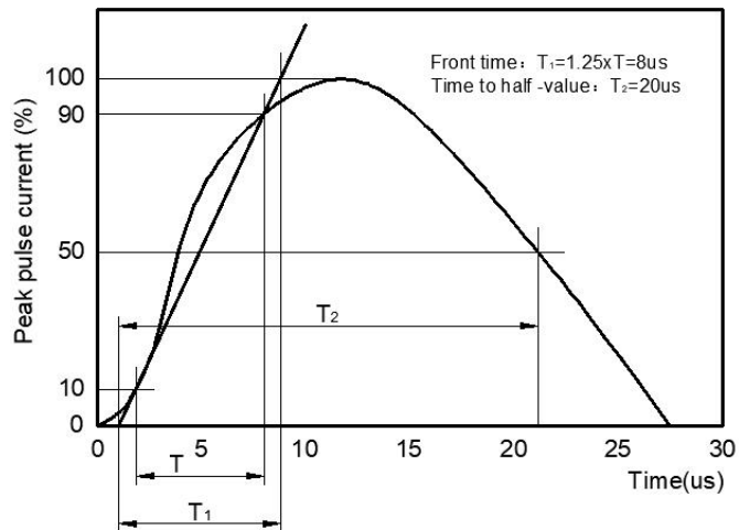
FIG2: pulse Waveform
