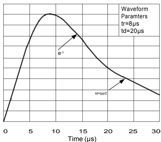
Figure3: Pulse Waveform
