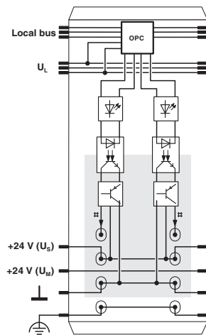
Block diagram
