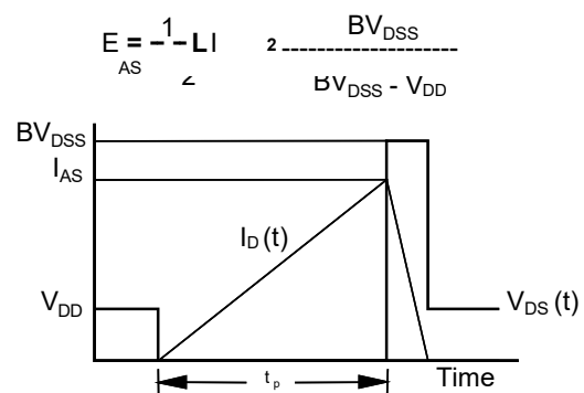
Unclamped Inductive Switching Test Circuit &amp; Waveforms
