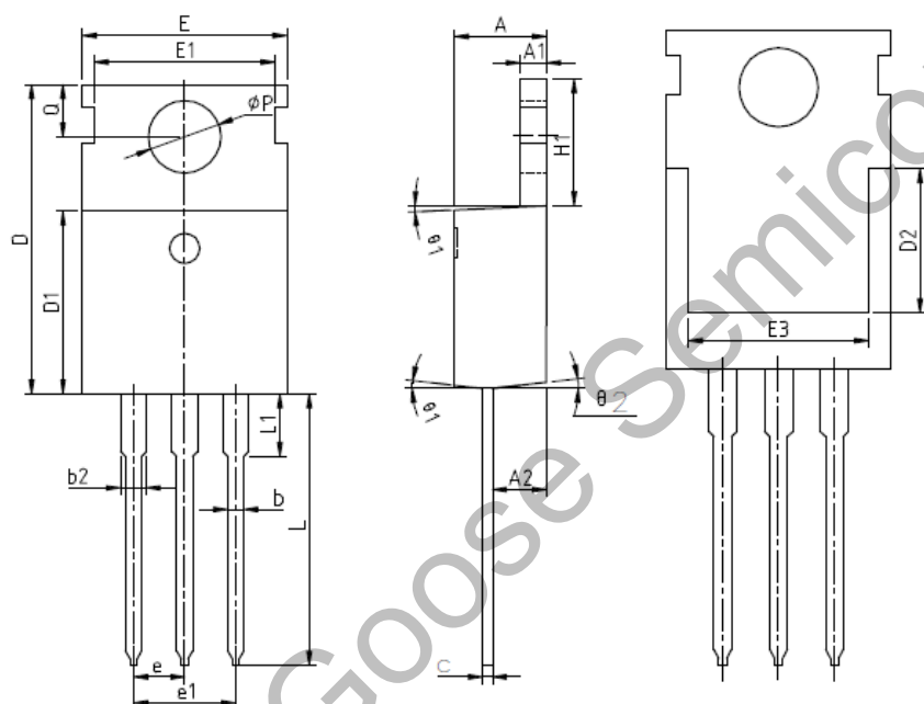
TO-220
