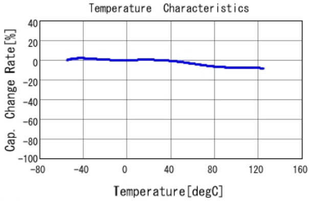
■ GCE188R71H332KA01 C-Temp. capchange, DCO. 0V, AC1. 0Vrm
