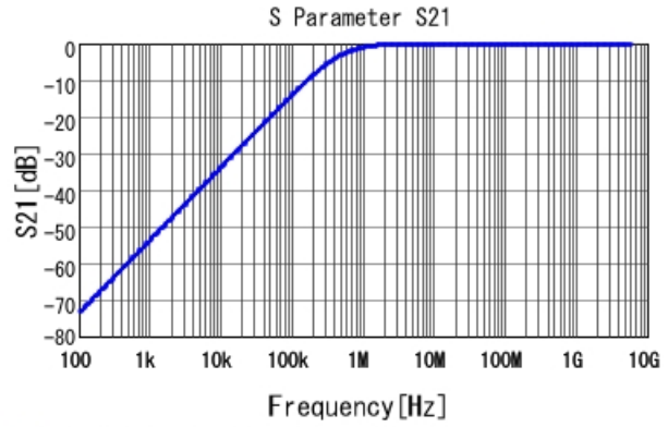
■ GCE188R71H332KA01 S21 DCOV, 25degC
