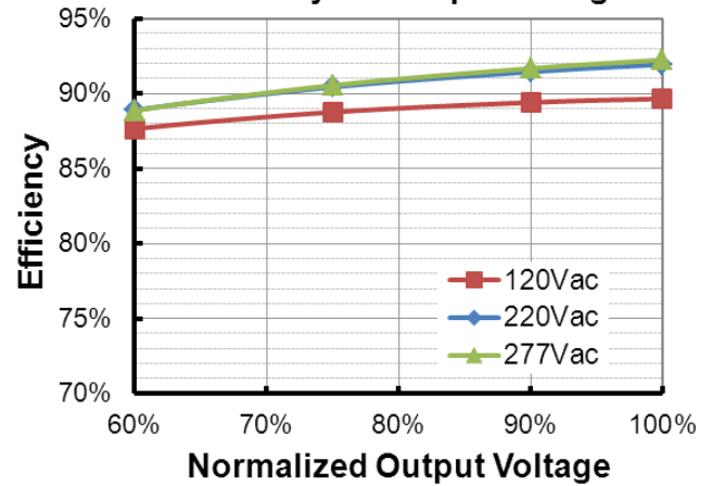
EUD-150S105DTL (I o =1050mA) Efficiency vs. Output Voltage
