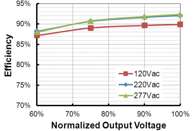
EUD-150S070DTL (I o =700mA) Efficiency vs. Output Voltage
