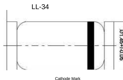
Glass case MiniMELF Dimensions in mm
