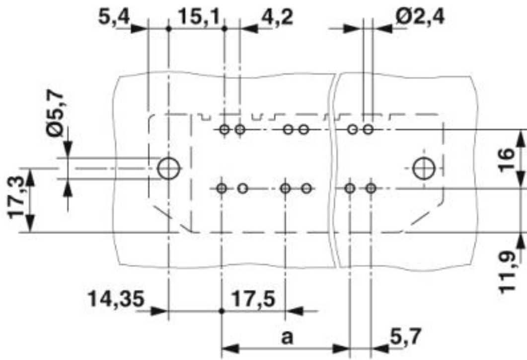
Drilling diagram
