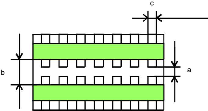
Fig.2 Substrate for temperature cycle test
