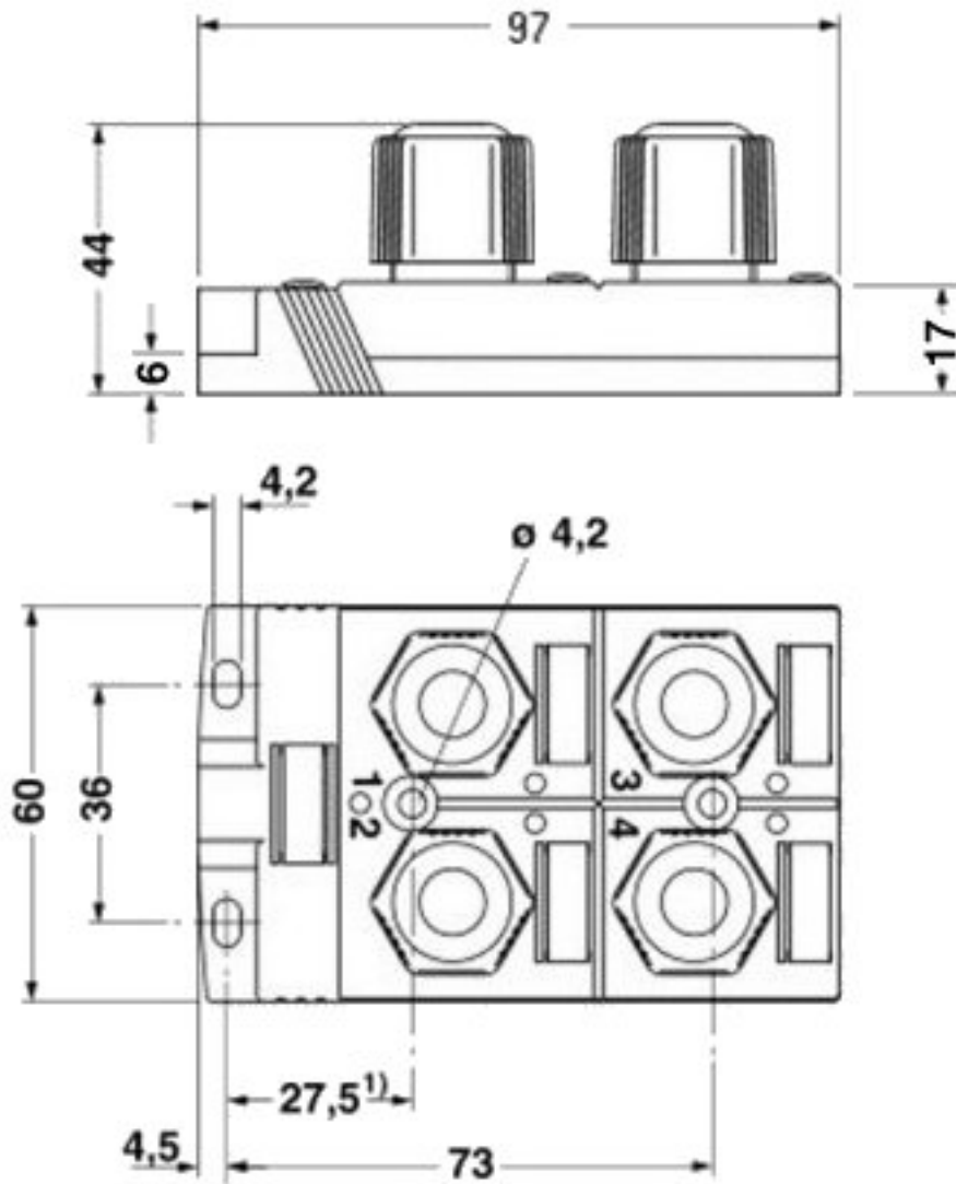
Dimensional drawing
