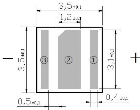
焊盘建议大小 Recommended size of pad
