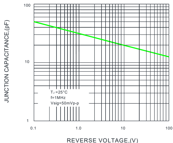
FIG.5-TYPICAL JUNCTION CAPACITANCE
