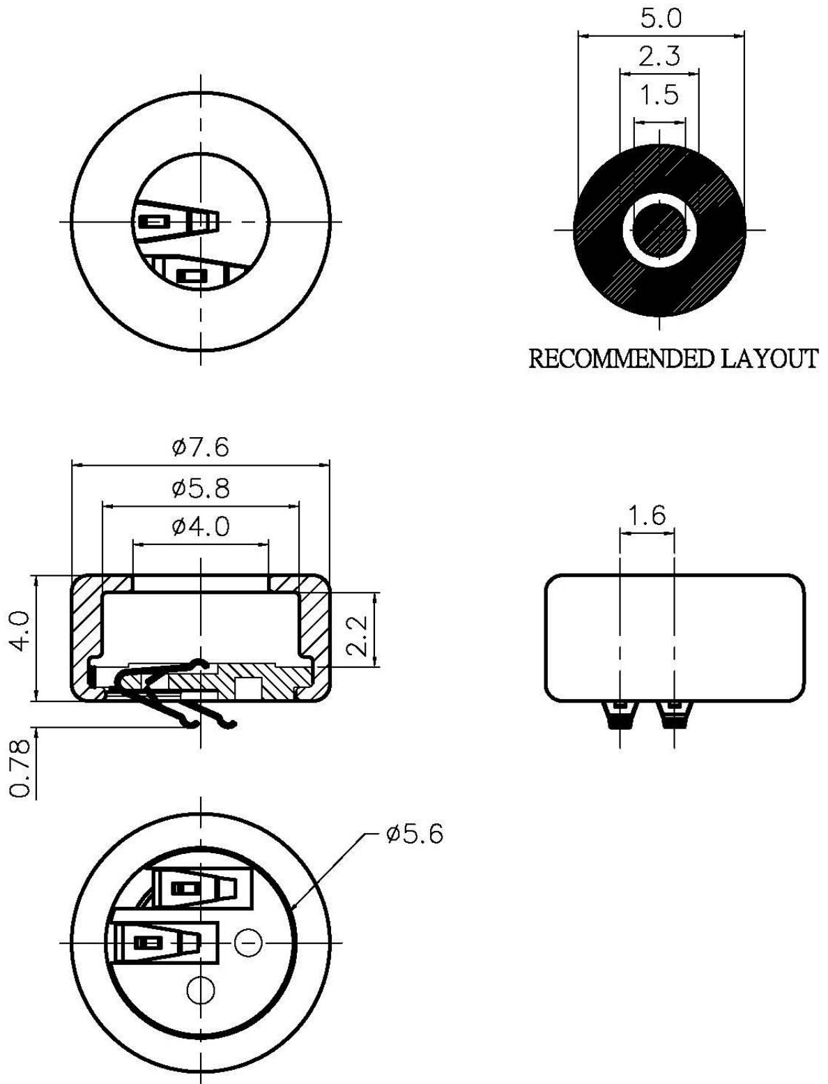
Fig D-2 Dimension of rubber holder
