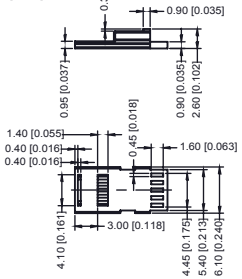
INSULATOR
