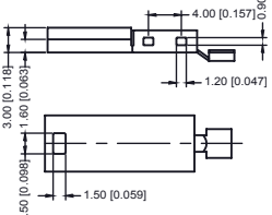
BOTTOM METAL SHELL
