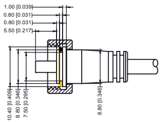
RECOMMENDED ASSEMBLY
