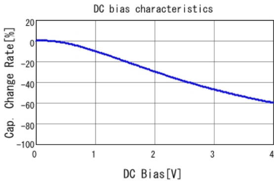
■ GRM188R60G106ME47 C-DC bias capchange, 25.0degC, AC0.
