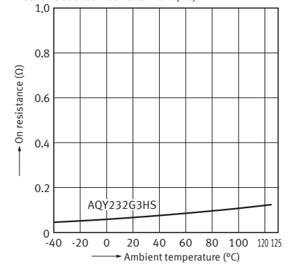
3-2. On resistance vs. ambient temperature characteristics
