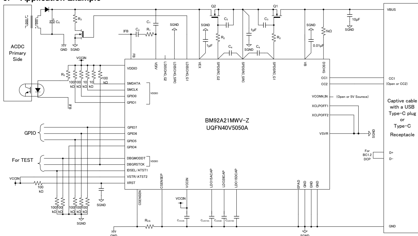
Figure 5-1 Application Example
