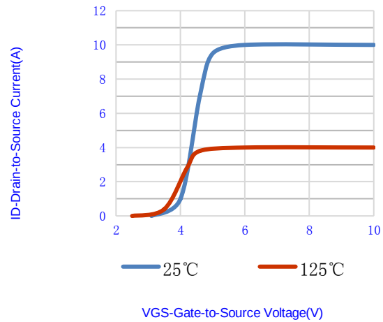
Fig.2- Transfer Characteristics
